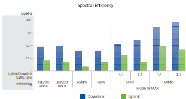
Figure 7. Mobile WiMAX vs. 3G Spectral Efficiency Comparison Source: WiMAX Forum [10].
