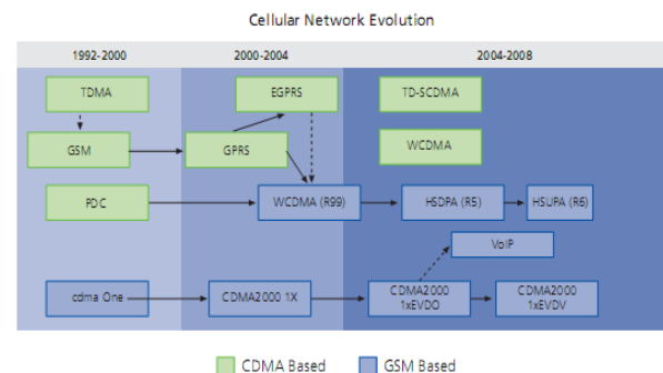
Figure 3. Cellular Network Evolution Source: Intel [2]
