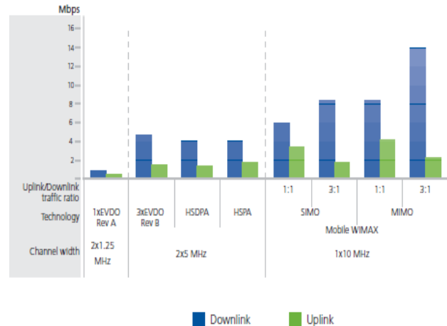
Figure 8. Mobile WiMAX vs. 3G Net Throughput Comparisons Source: WiMAX Forum [9].
