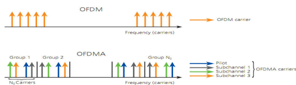
Figure 1: Single Carrier and OFDMA received Signals
