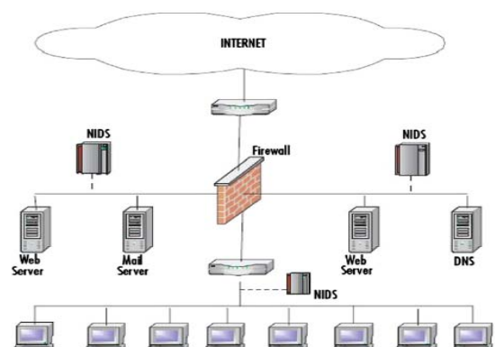
Figure 4. Network Based Intrusion Detection System (NIDS)
