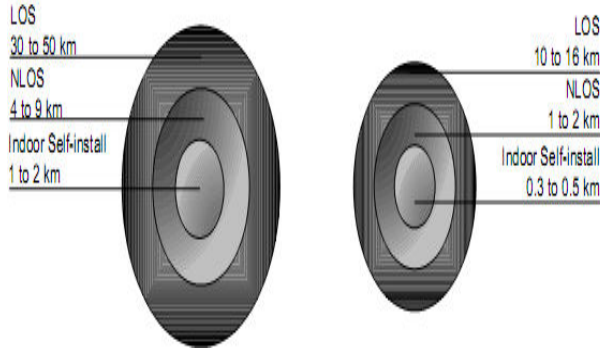
Figure. 8. Full featured and standard cell radii
