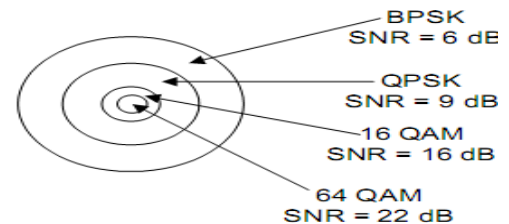
Relative cell radii for adaptive modulation
