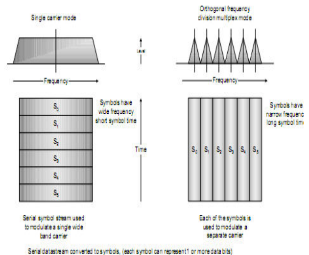
Figure 4. Single carrier and OFDM
