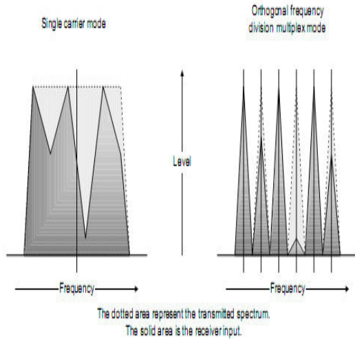
Figure. 5. Single carrier and OFDM received signals
