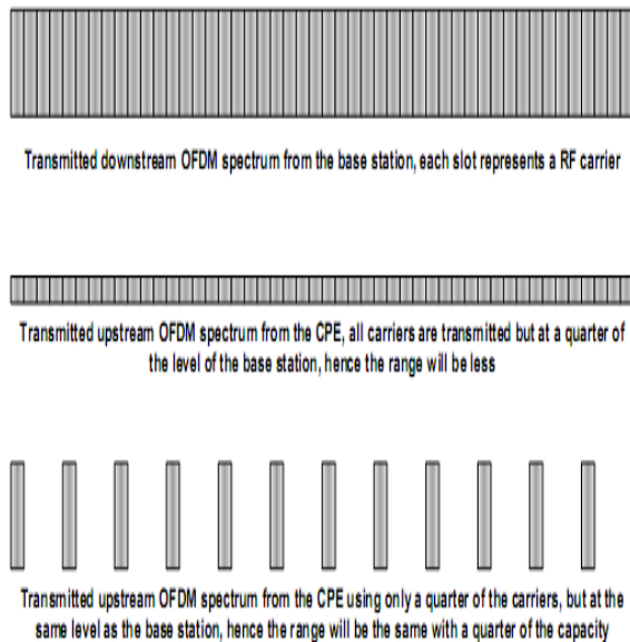
Figure. 6. The effect of sub-channelization
