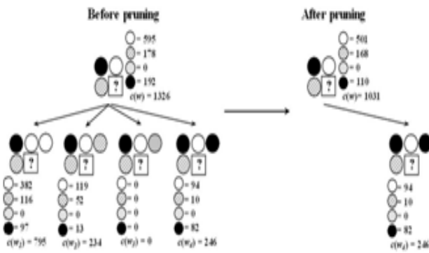
Figure. 4. Example of a single-node pruning: Resulted node configuration is (0,0,0,1).
