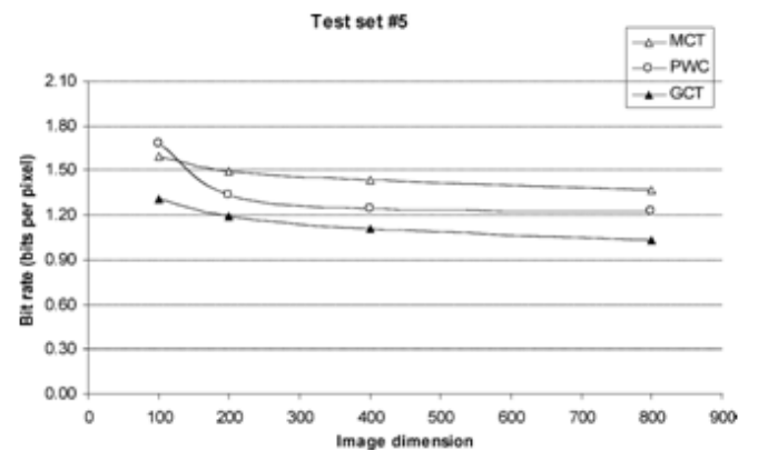
Figure. 10. Dependency of the bit rate on the image size.
