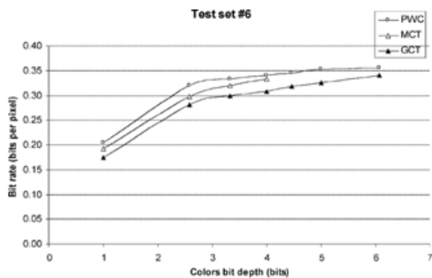
Figure. 11. Dependency of the bit rate on the image color depth.
