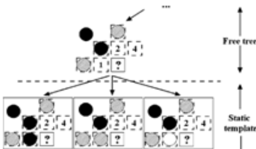
Figure. 8. Example of the hybrid tree: Locations of depths less than or equal to four are defined by the free tree, and locations of bigger depth are defined by unused positions in the static template.
