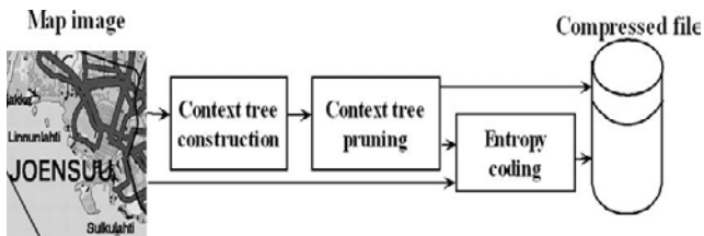
Figure 2. Overall scheme of the proposed algorithm.
