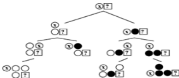
Figure. 7. Illustrative example of the free tree.
