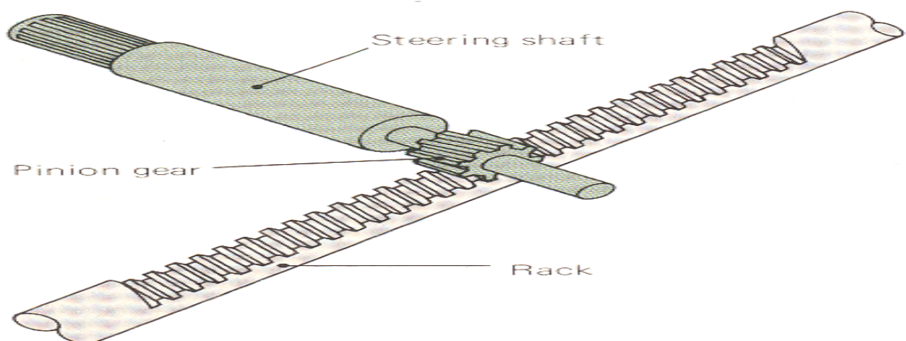
Figure 4: Rack and pinion arrangement
