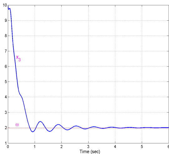
Figure 4. Constant Tracking Problem for x_3
