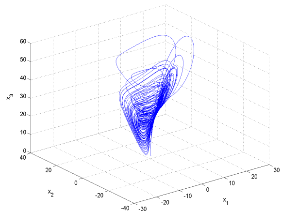
Figure 1. State Orbits of the Unforced Chen System
