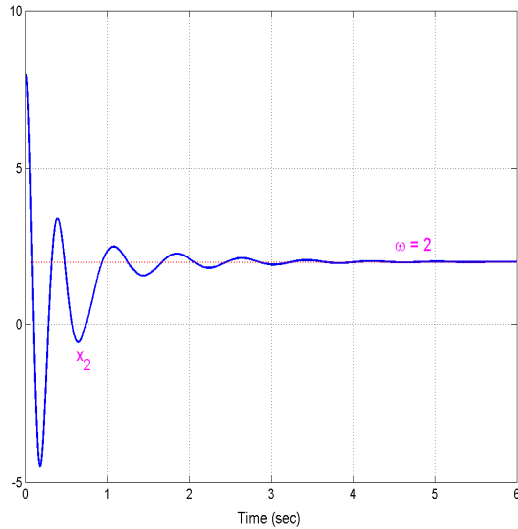
Figure 3. Constant Tracking Problem for x_2
