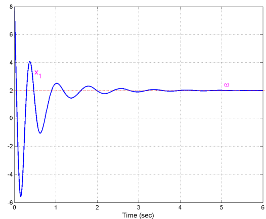
Figure 2. Constant Tracking Problem for x_1
