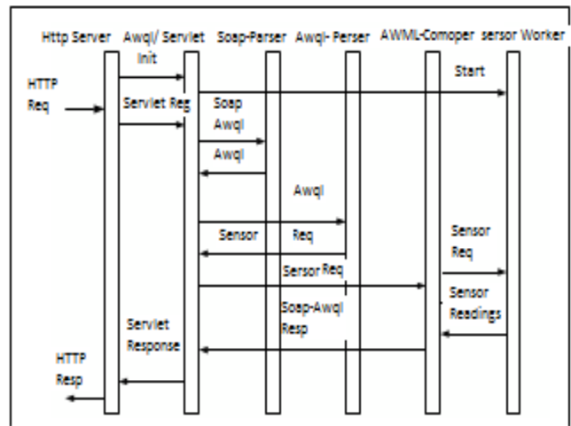
Figure 5: Overview of the query process
