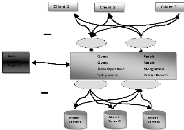
Figure 1: The Nexus Architecture
