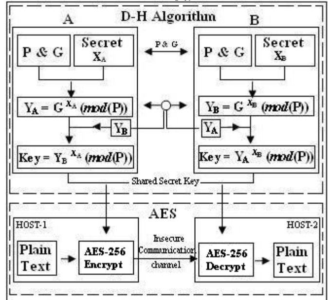
Figure. 2 New network based security model.
