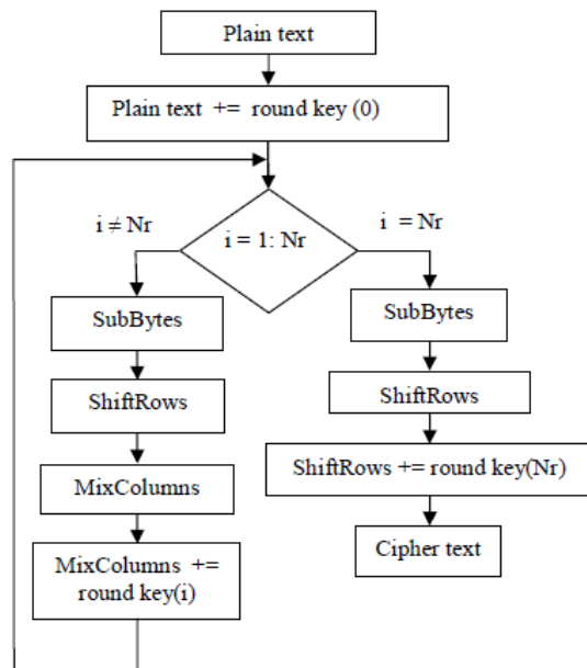
Figure 1 AES Encryption Algorithm
