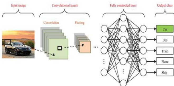
Figure1: CNN image classification pipeline [8].
